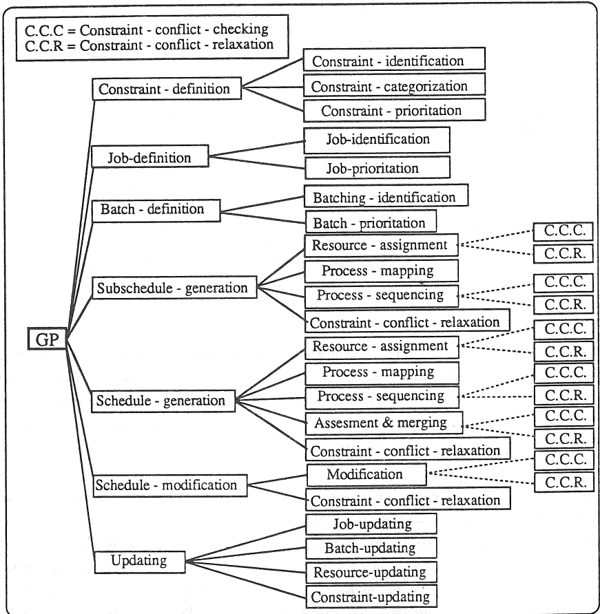
Figure 2-2. Experimentl generic processes for scheduling.
