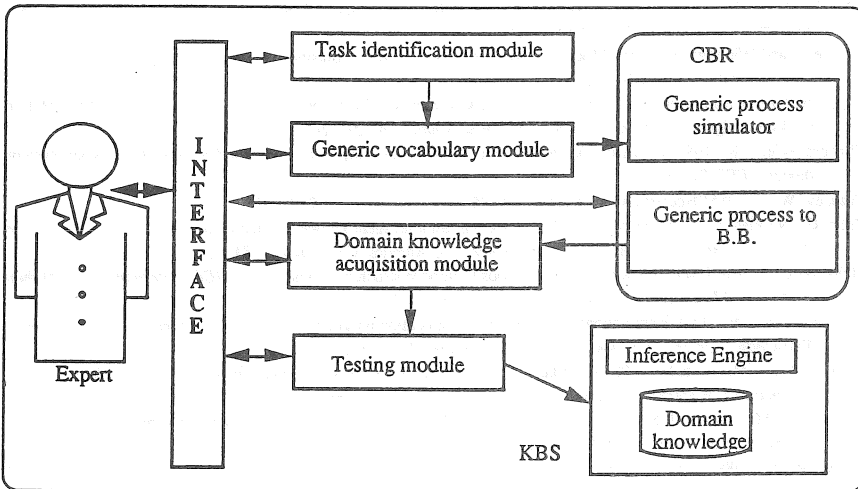
Figure 4-1. Multis Architecture.
