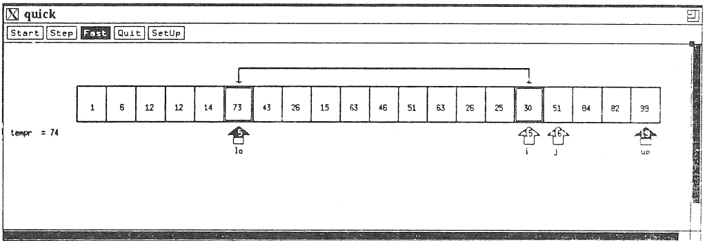
Figure 4: Debugging mode.
