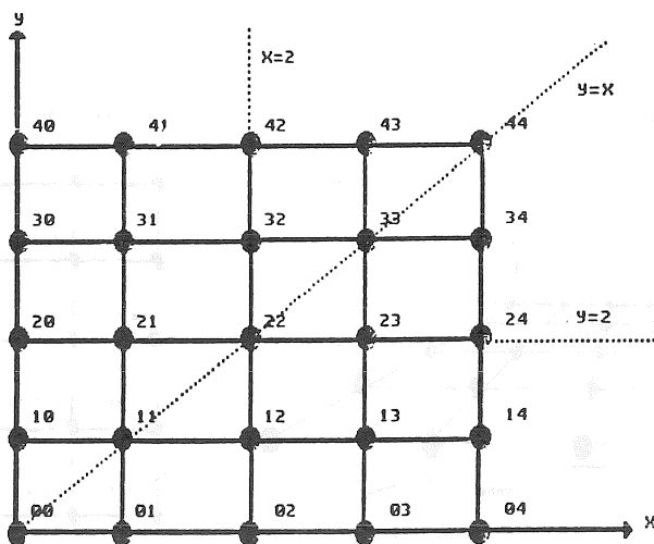
Figure 3. Symmetry axes in the initial implementation of the LU decomposition implementation
