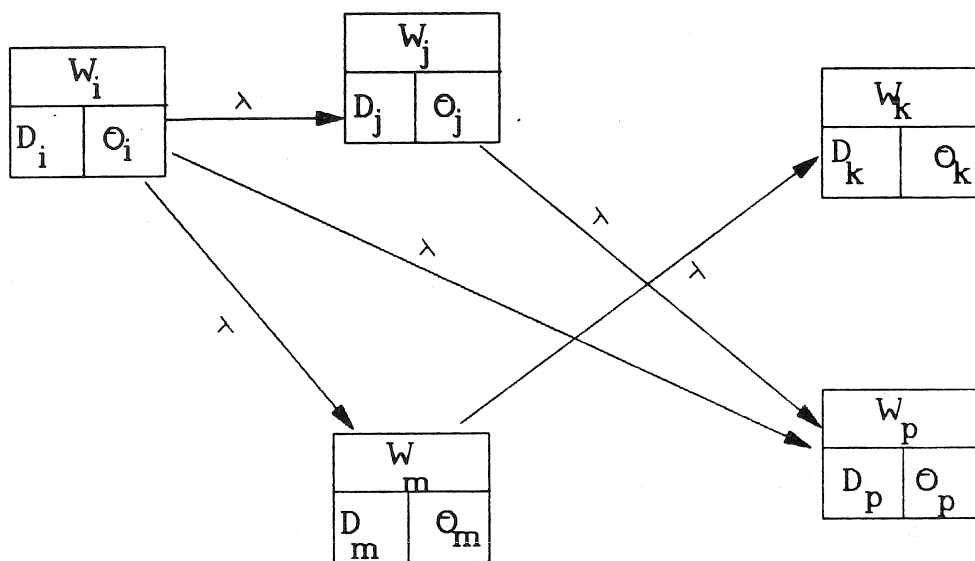
Fig.1 Connectionist model
